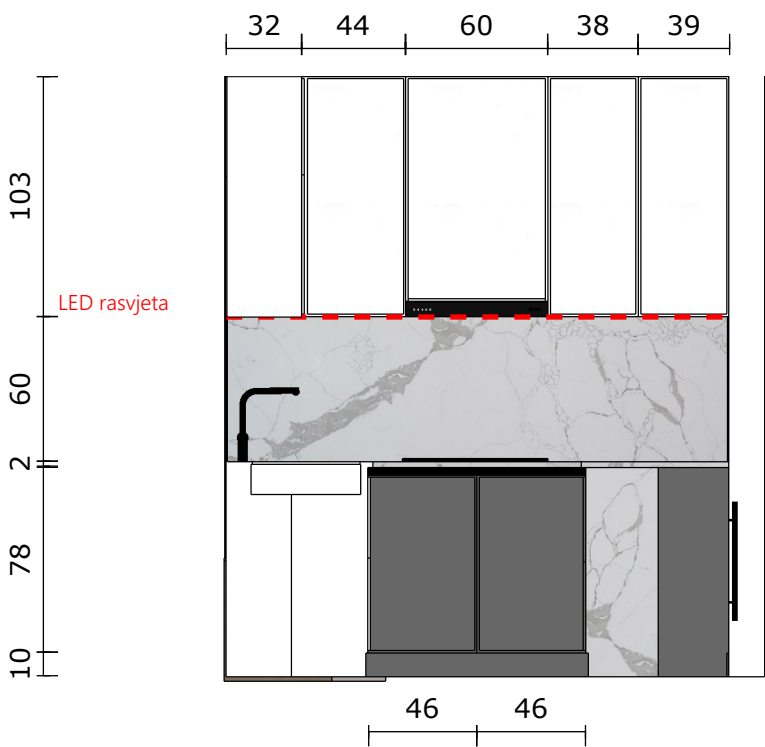
Pogled B_B
